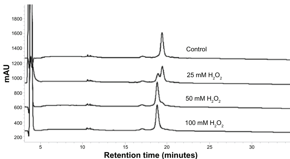
Figure 7 Effect of increasing the concentration of H 2 O 2 on the RP-HPLC profile of a pneumococcal vaccine antigen.
